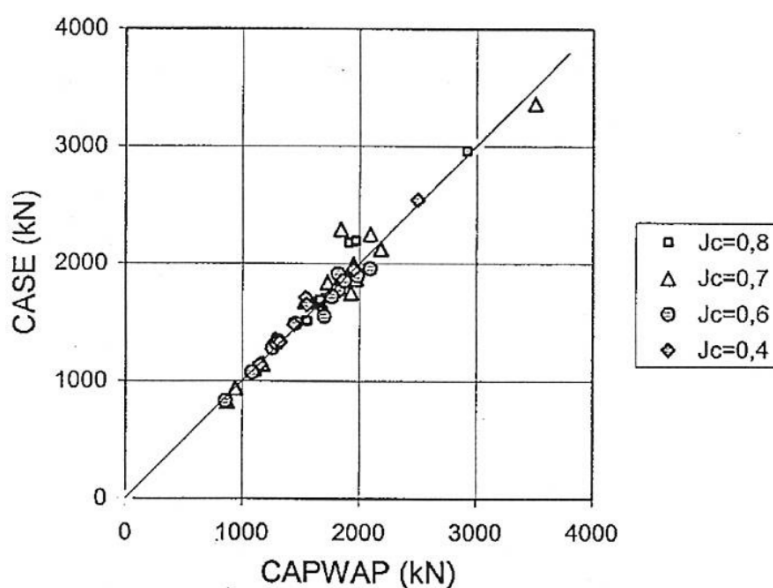
Figure 7: Correlation between CAPWAP and the Case-method for driven end-bearing piles according to Axelsson et al. (2004).
